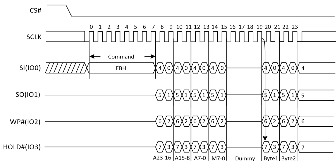
Figure 12. Quad I/O Fast Read Sequence Diagram (M5-4≠(1, 0))
