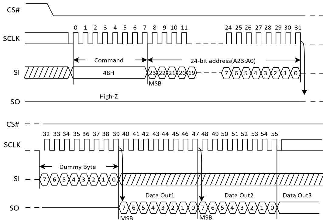
Figure 29. Read Security Registers command Sequence Diagram
