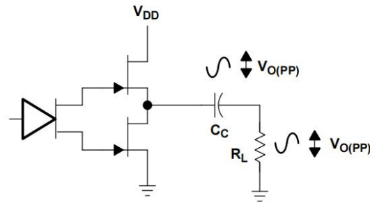
Figure 35. Single-Ended Configuration
