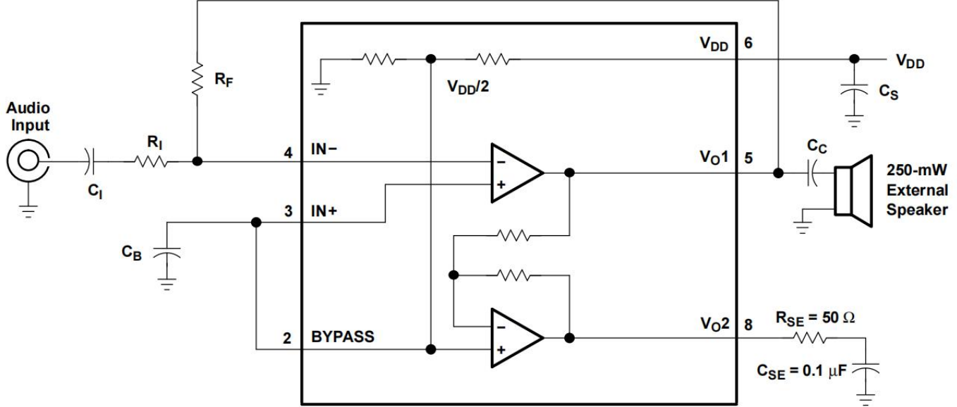
Figure 38. Singled-Ended Mode
