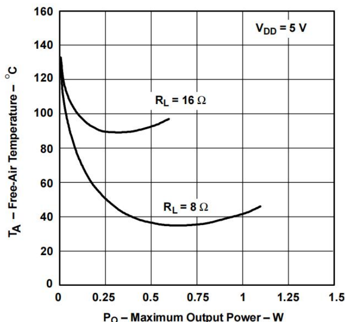
Figure 39. Free-Air Temperature vs Maximum Continuous Output Power
