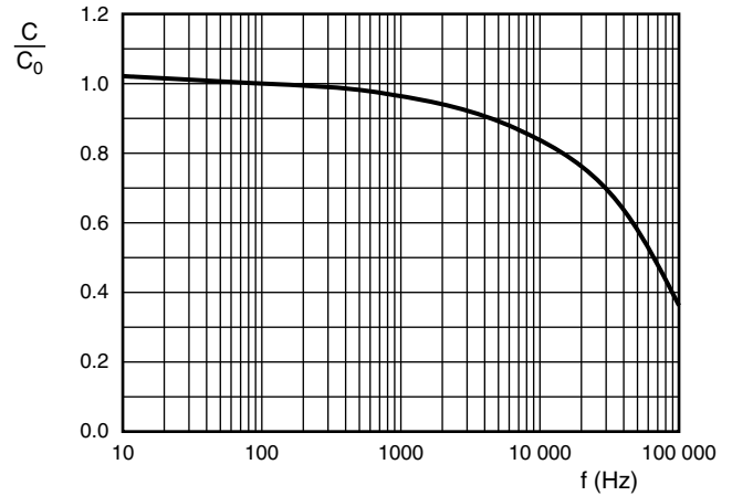
Fig. 6 - Typical multiplier of capacitance as a function of frequency at 20 ^{\circ}\text{C} ( C_0 = C at 100 Hz)
