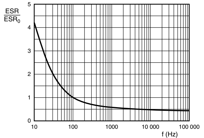
Fig. 8 - Typical multiplier of ESR at 20 ^{\circ}\text{C} as a function of frequency ( \text{ESR}_0 = \text{ESR} at 100 Hz)
