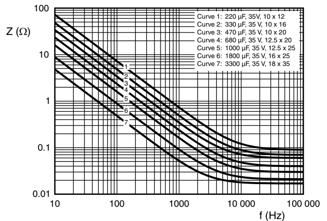
Fig. 10 - Typical impedance Z at 20 ^{\circ}\text{C} as a function of frequency
