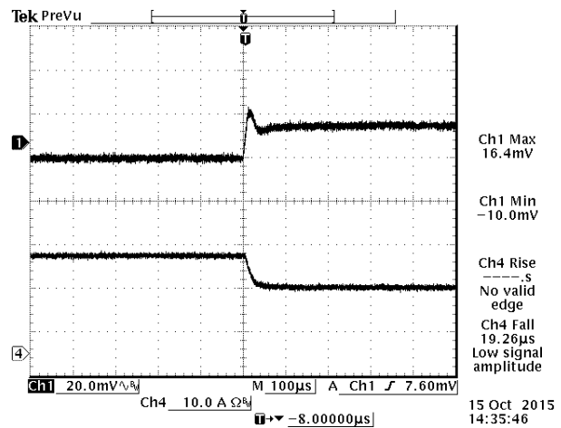
Figure 12. Vin= 75% - 50% Load Transient at Vin = 12 VDC Vout = 0.9 VDC @Ta=25 °C
