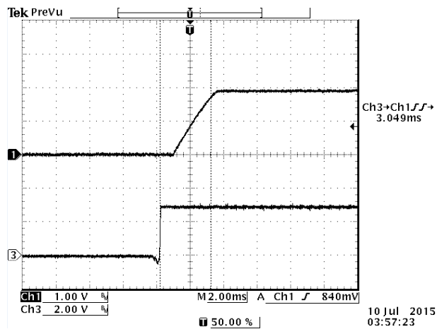
Figure 20. Start up time at full load, 12VDC input 2.0VDC/30A output and T_a=25^\circ\text{C}
