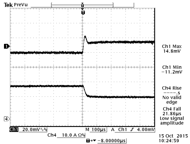
Figure 10. Vin= 75% - 50% Load Transient at Vin = 12 VDC Vout = 0.6 VDC @Ta=25 °C
