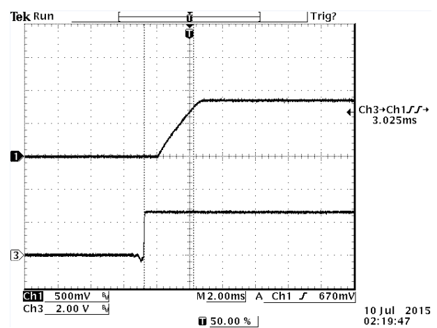
Figure 19. Start up time at full load, 12VDC input 0.9VDC/30A output and T_a=25^\circ\text{C}
