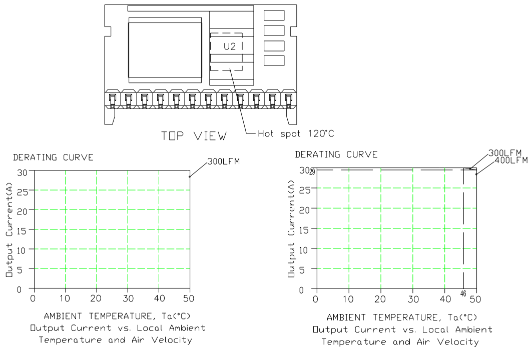
Figure 3. V_{in} = 12V , .06V \leq V_o < 1.2V
