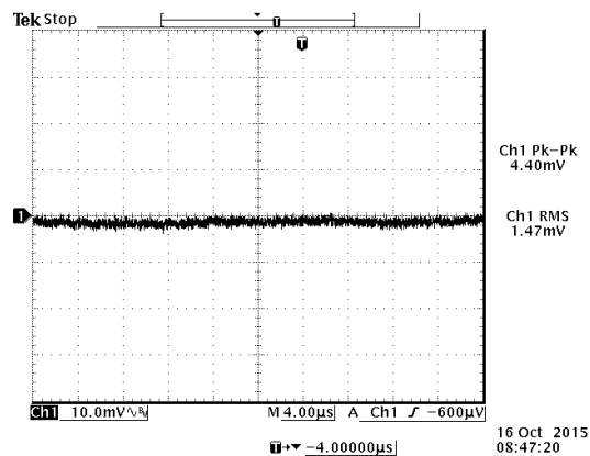
Figure 8. Ripple and noise at full load, 12VDC input 2.0VDC/30A output and Ta=25 °C
