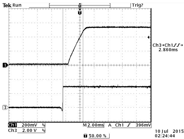
Figure 18. Start up time at full load, 12VDC input 0.6VDC/30A output and T_a=25^\circ\text{C}
