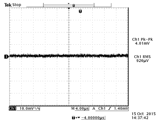
Figure 7. Ripple and noise at full load, 12VDC input 0.9VDC/30A output and Ta=25 °C
