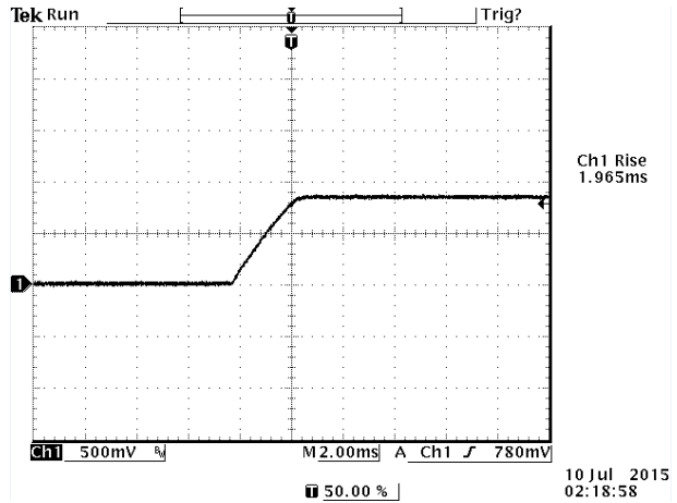
Figure 16. Rise time at full load, 12VDC input 0.9VDC/30A output and T_a=25\text{ }^{\circ}\text{C}
