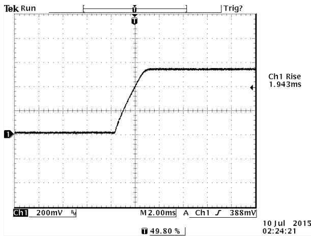
Figure 15. Rise time at full load, 12VDC input 0.6VDC/30A output and T_a=25\text{ }^{\circ}\text{C}
