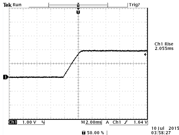
Figure 17. Rise time at full load, 12VDC input 2.0VDC/30A output and T_a=25\text{ }^{\circ}\text{C}
