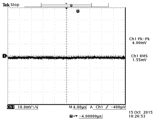
Figure 6. Ripple and noise at full load, 12VDC input 0.6VDC/30A output and Ta=25 °C
