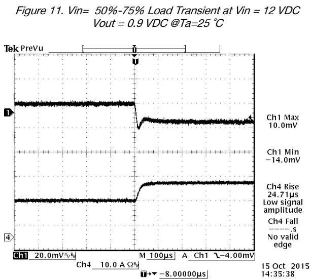
Figure 11. Vin= 50%-75% Load Transient at Vin = 12 VDC Vout = 0.9 VDC @Ta=25 °C
