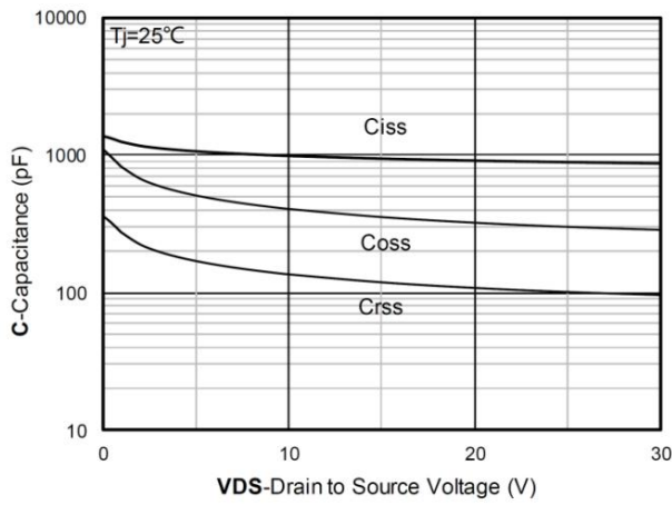
Capacitance Characteristics
