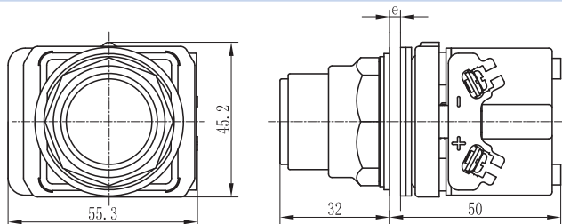
PB(M)30-MP
