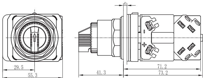
PB(M)30-S
