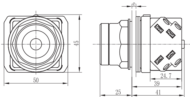
PB(M)30-MIP
