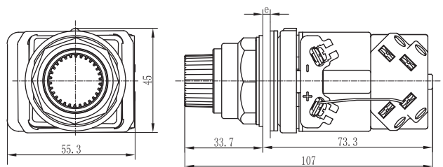
PB(M)30-PTL
