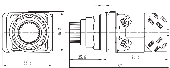
PB(M)30-PTL
