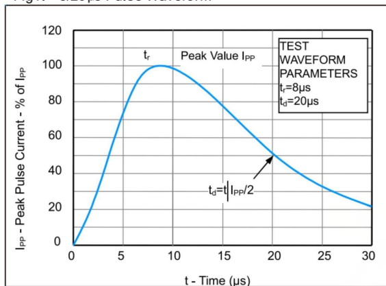
Fig1. 8/20 \mu\text{s} Pulse Waveform
