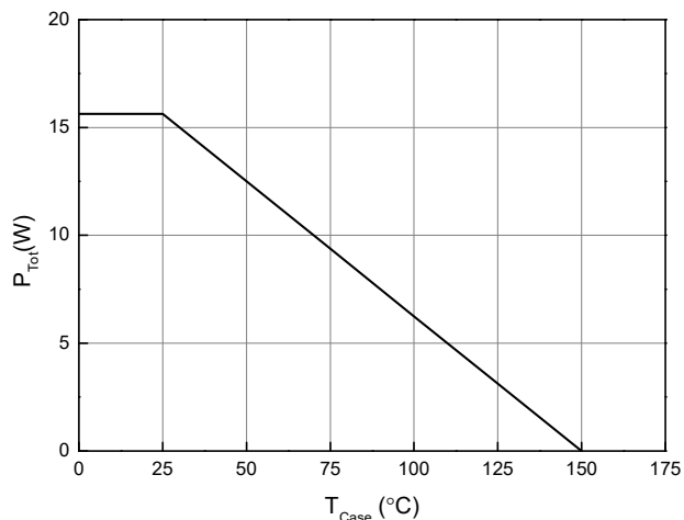
Figure 9. Power Dissipation
