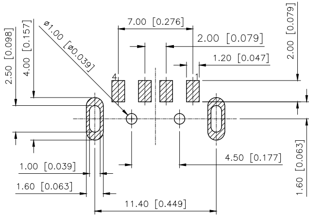
PCB_LAYOUT
