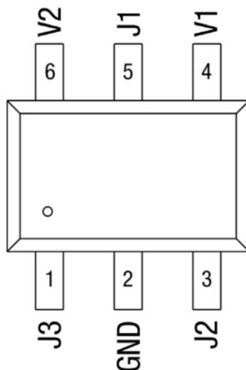
Figure 2. XA214-G4C Pinout (Top View)
