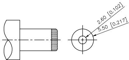
MATING PLUG Jack Insertion Depth: 8.2 mm
