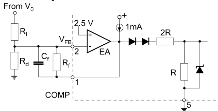
Figure 5. Latched Shutdown
