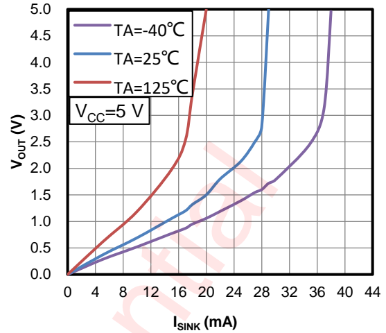
Figure 12 V_{OUT} vs. I_{SINK}
