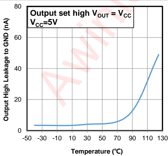
Figure 15 I_{OH} vs. Temperature
