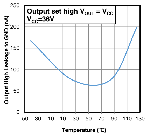
Figure 16 I_{OH} vs. Temperature
