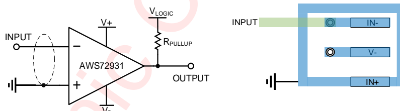
Figure 25 Inverting Comparator Application Schematic and Layout Example
