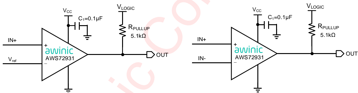
Figure 21 Single-Ended and Differential Comparator Configurations
