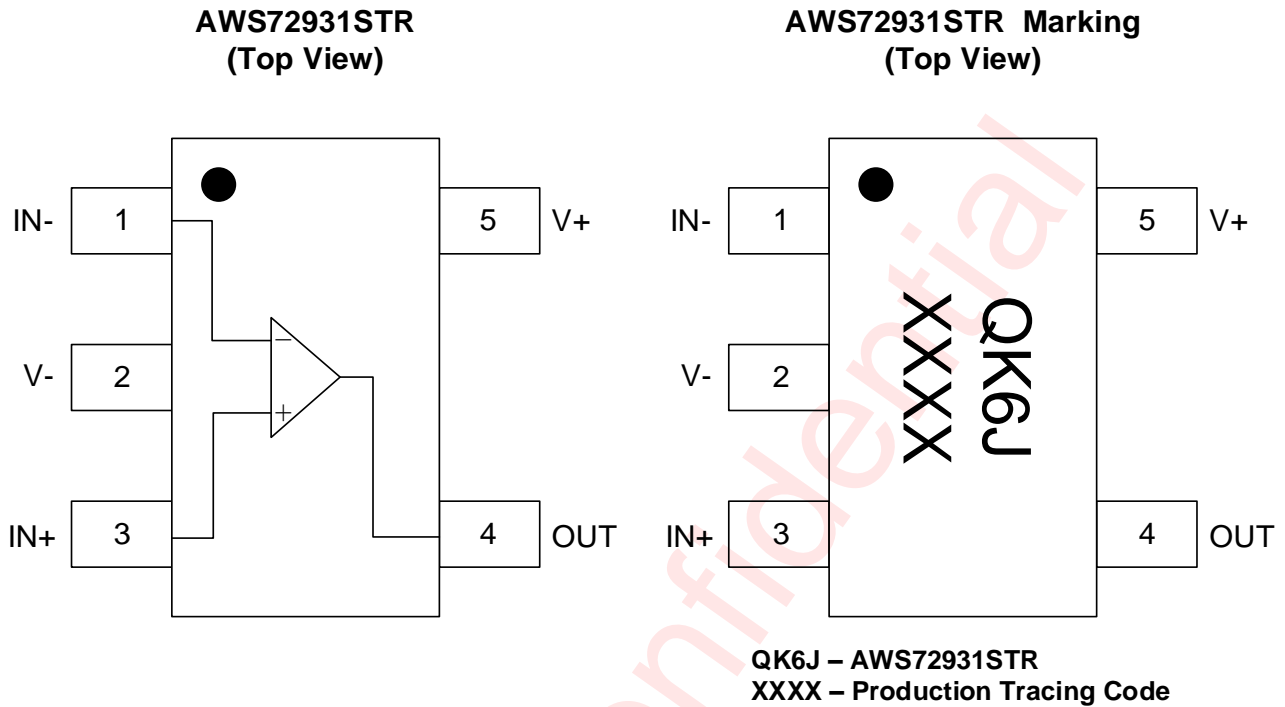
Figure 2 Pin Configuration
