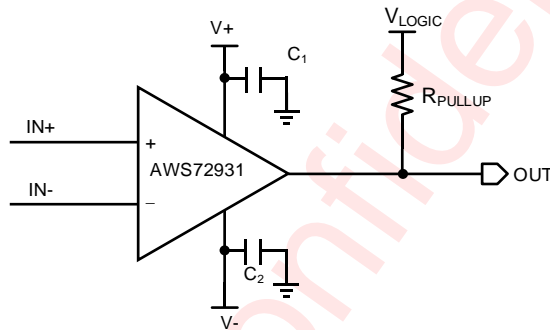
Figure 22 AWS72931 Schematic Example
