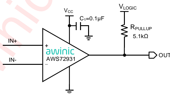
Figure 4 AWS72931 Application Circuit
