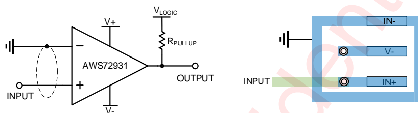
Figure 24 Non-inverting Comparator Application Schematic and Layout Example
