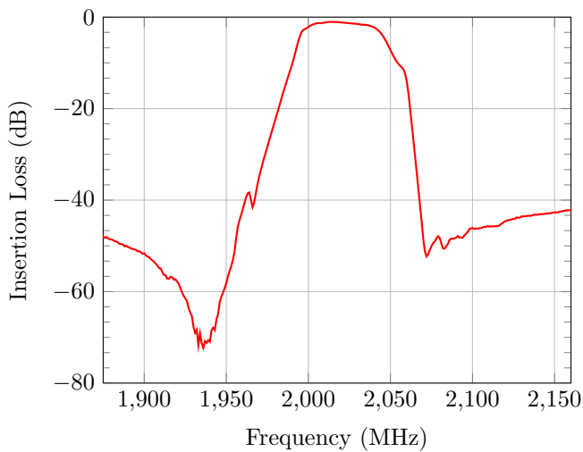
Figure 6: Narrowband
