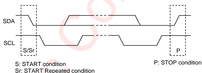
Figure 77 I 2 C Start/Stop Condition Timing
