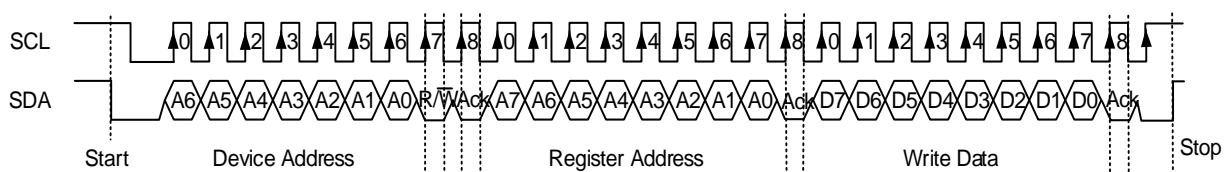
Figure 80 I 2 C Write Byte Cycle
