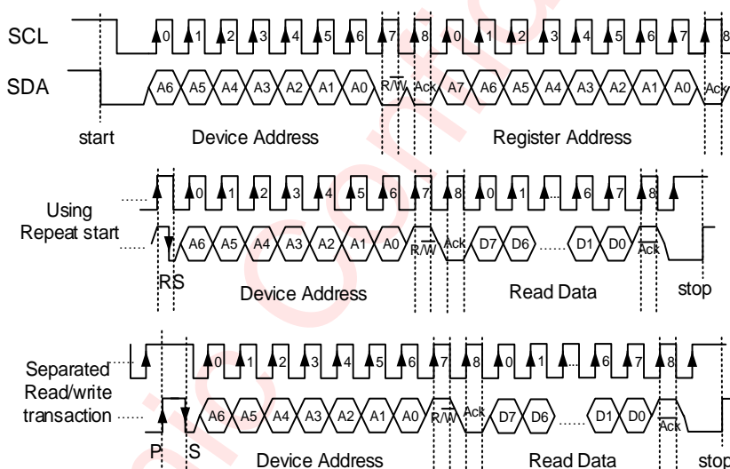
Figure 81 I 2 C Read Byte Cycle
