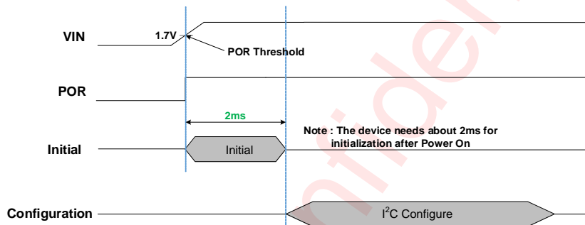
Figure 75 Power Up Timing
