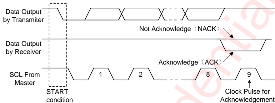
Figure 79 I 2 C ACK Timing
