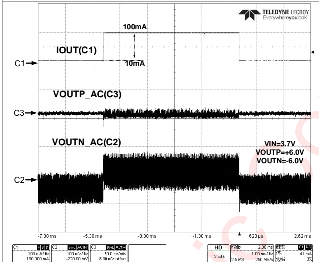
Figure 55 Load Transient (100mA Mode)
