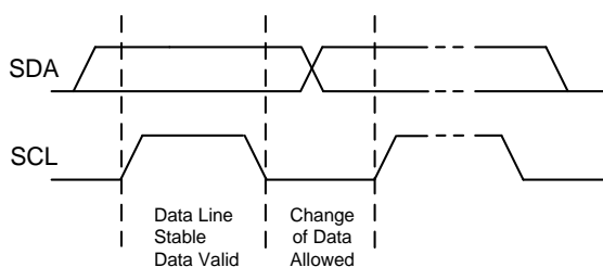
Figure 78 Data Validation Diagram
