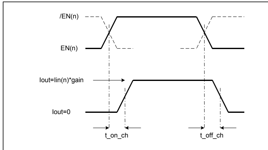
Figure 25 - Timing of Read or Write Channels
