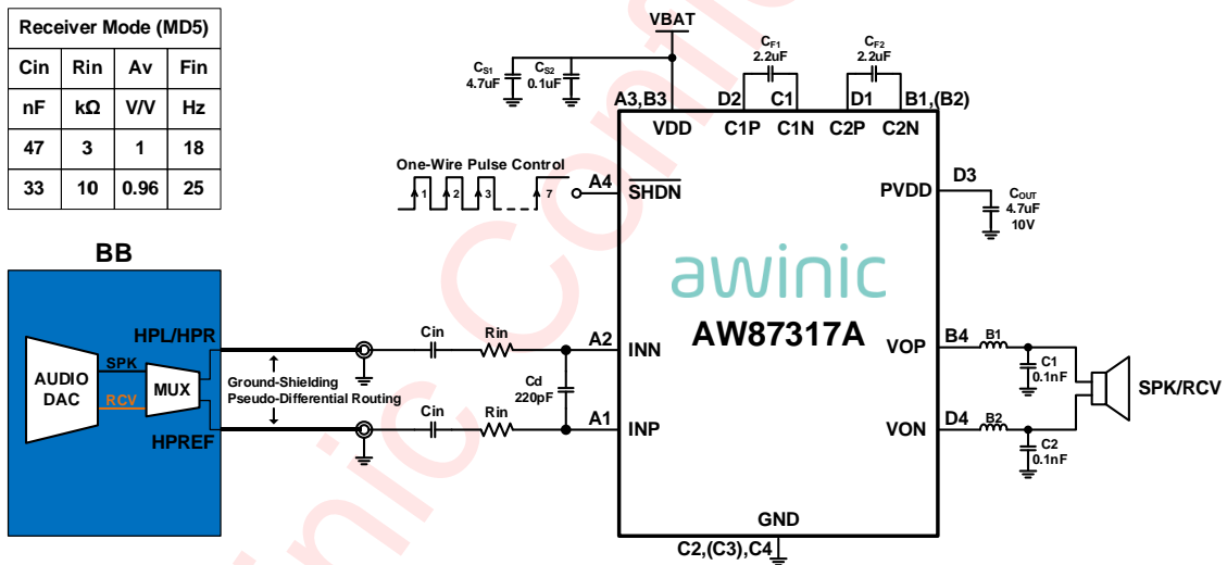
Figure 5 AW87317A Receiver Mode Application Diagram
