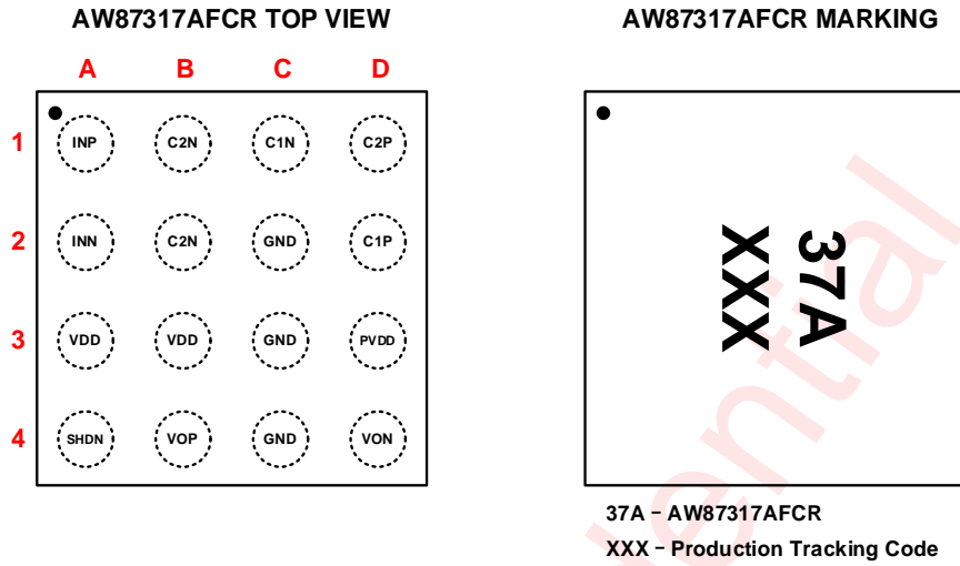
Figure 2 AW87317A Pin Diagram Top View and Device Marking
