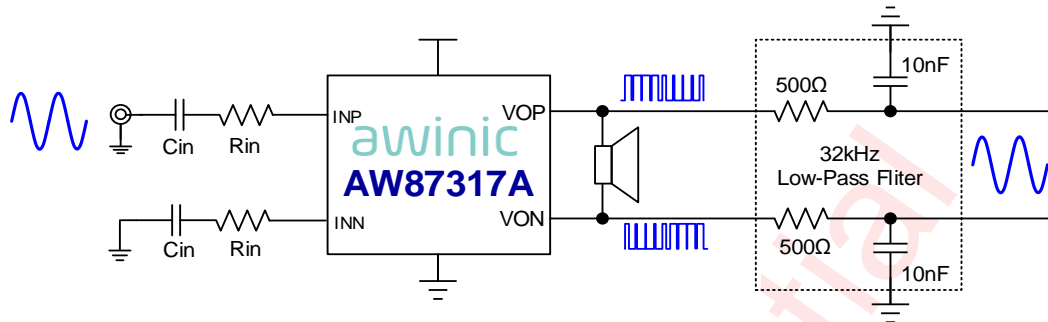
Figure 6 AW87317A Test Setup
