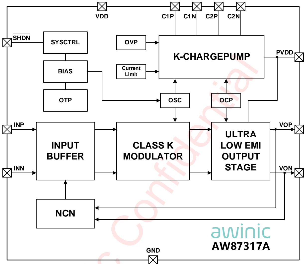
Figure 3 AW87317A Functional Diagram
