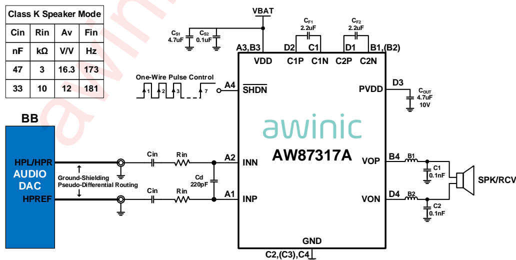
Figure 1 AW87317A Application Diagram
