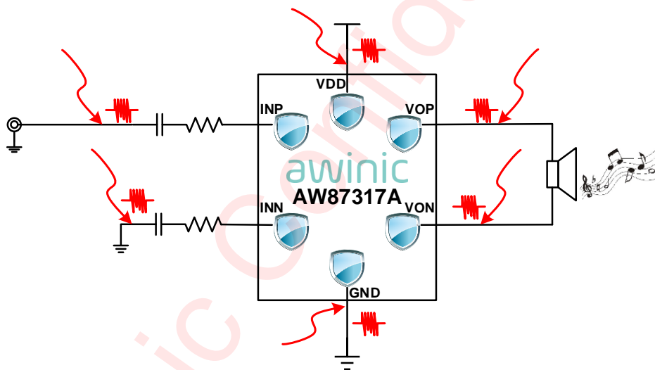
Figure 16 AW87317A Rejection of RF Noise
