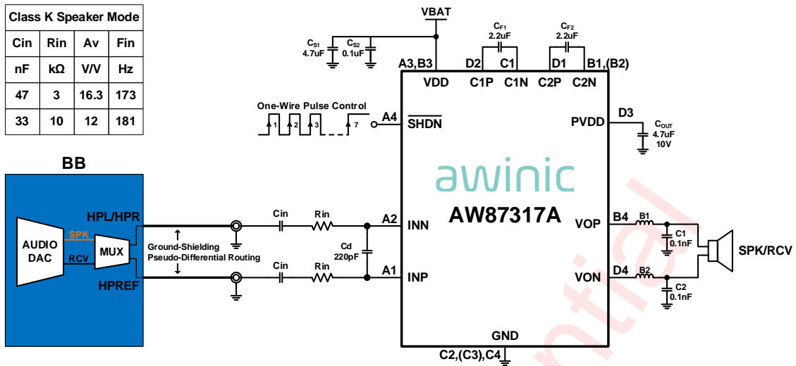
Figure 4 AW87317A Speaker Mode Application Diagram (Note 1)
