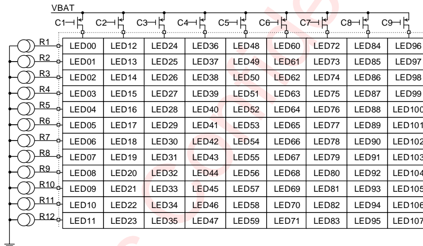
Figure 17 LED Location
