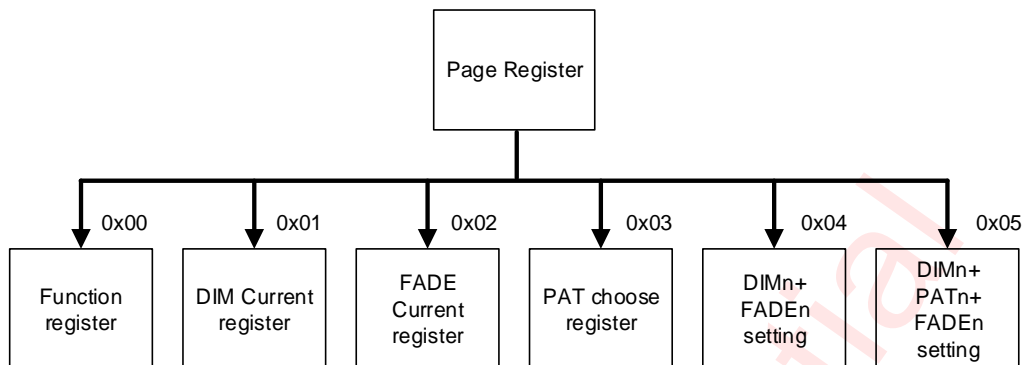
Figure 22 Register Control
