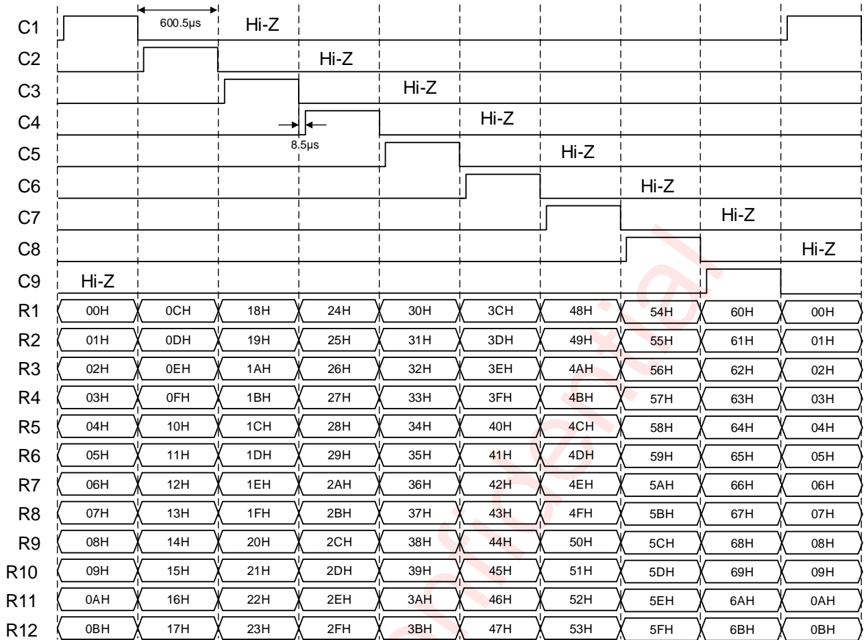
Figure 15 Scan Drive Operation of AW20108
