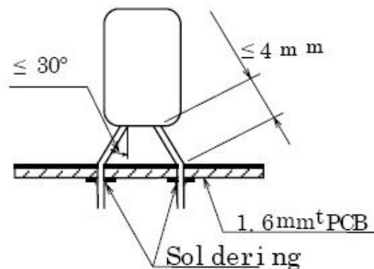
Fig. 4 Vibration test
