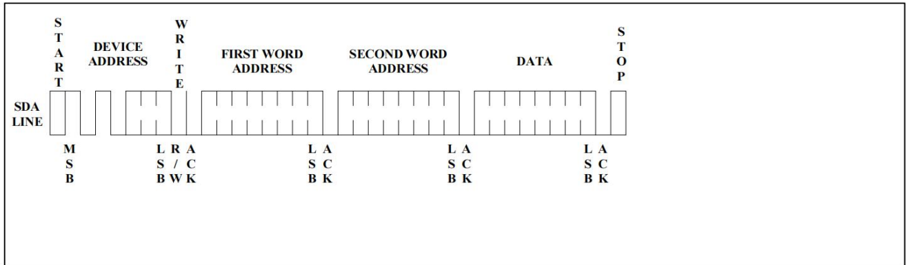
Figure 6. Byte Write
