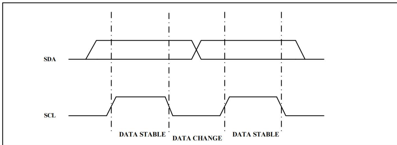
Figure 2. Data Validity
