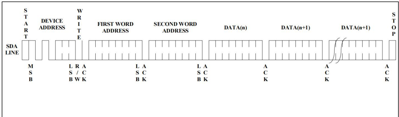
Figure 7. Page Write
