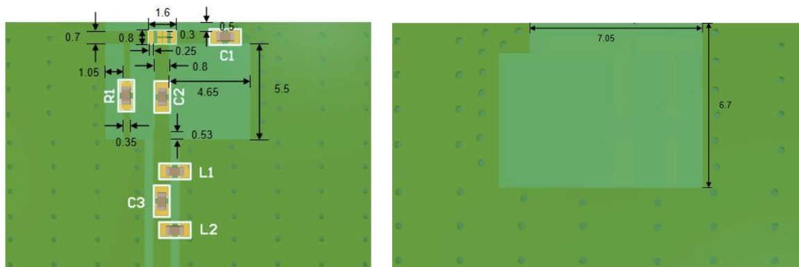
Figure 4. PCB Antenna Layout (Unit: mm)
