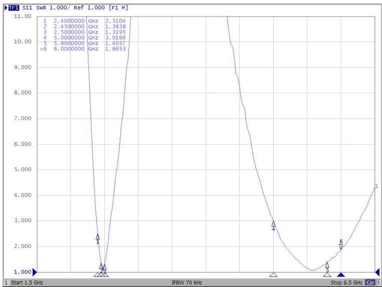
Figure 6. VSWR
