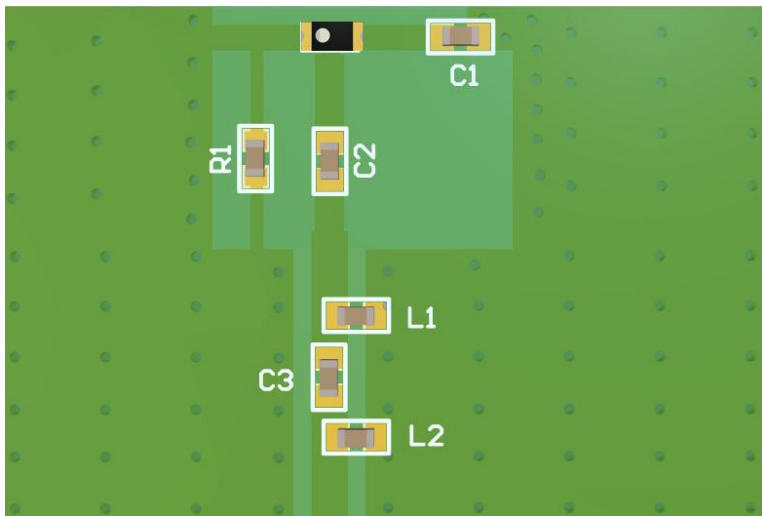
Figure 5. Matching Circuit (Unit: mm)
