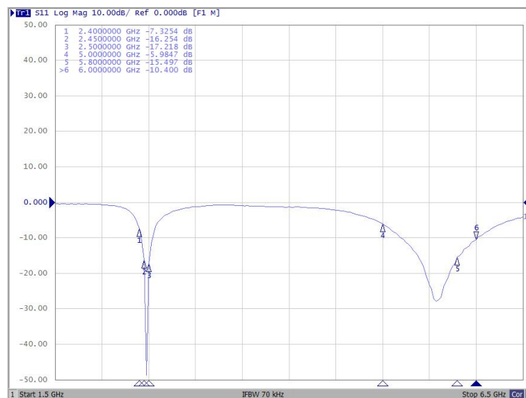
Figure 7. Return Loss
