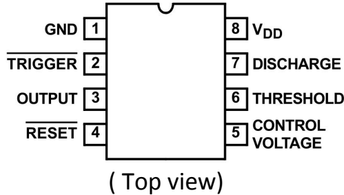
Pin Configuration
