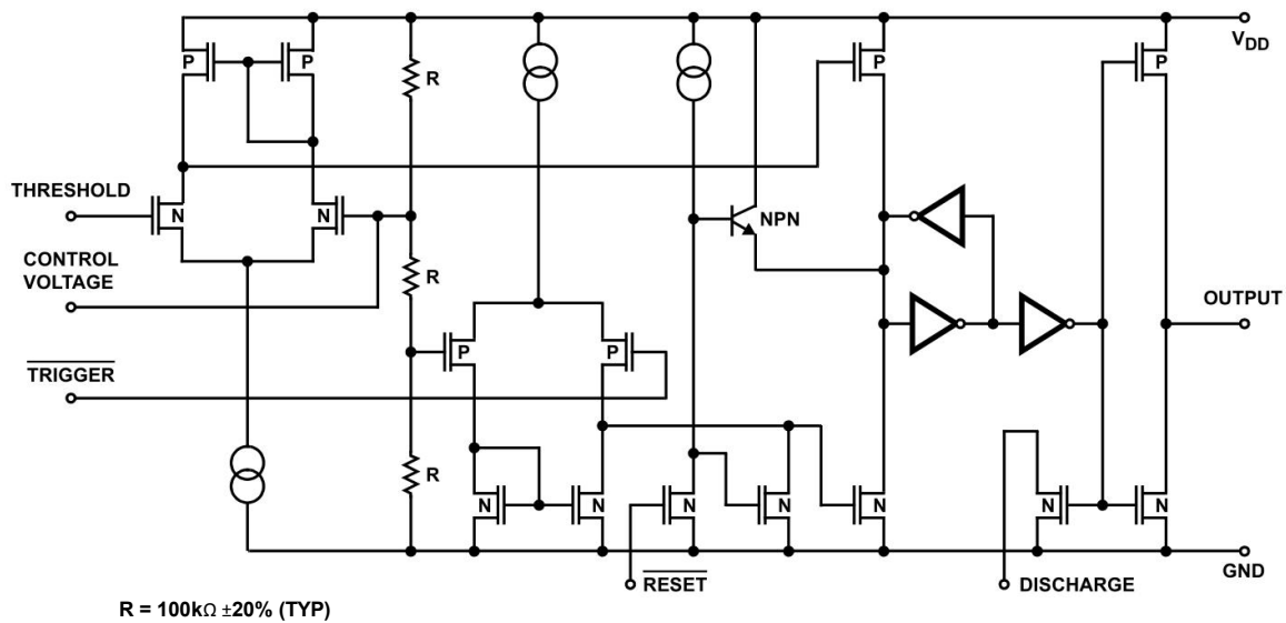
FIGURE 2. SCHEMATIC DIAGRAM
