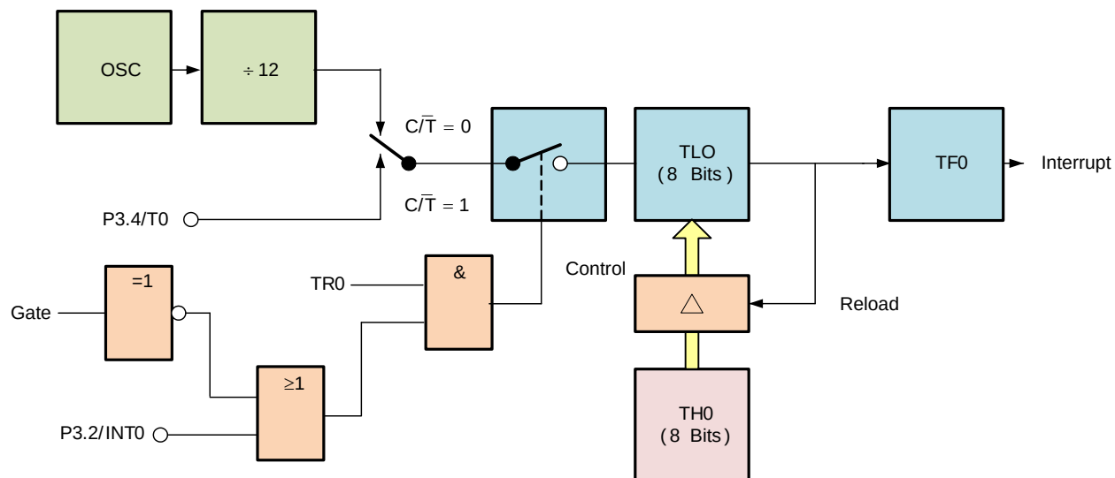
Figure 9. Timer 0 Mode 2
