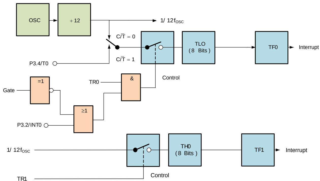
Figure 10. Timer 0 Mode 3
