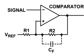
Figure 24. Configuring the AD8611/AD8612 with Hysteresis
