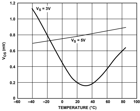
Figure 13. Offset Voltage vs. Temperature
