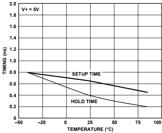
Figure 15. Latch Setup and Hold Time vs. Temperature
