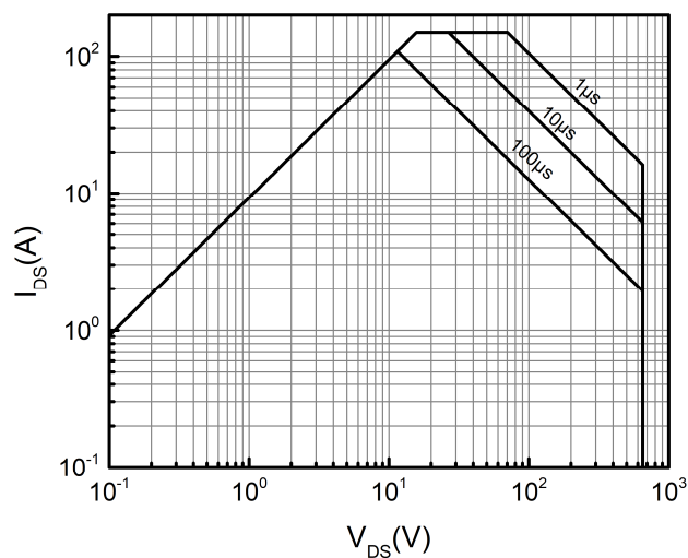
Figure 11. Safe Operating Area at T_C = 25°C
