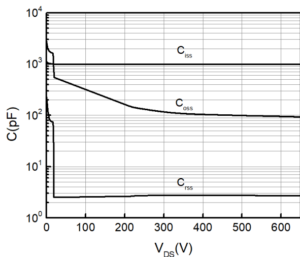
Figure 5. Typical Capacitance ( V_{GS} = 0V , f = 500kHz )
