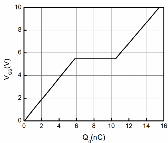
Figure 7. Typical Gate Charge ( I_{DS} = 22A , V_{DS} = 400V )
