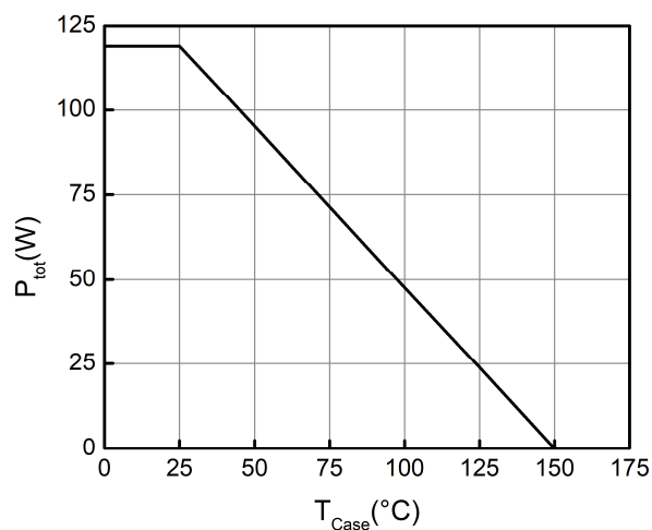
Figure 9. Power Dissipation
