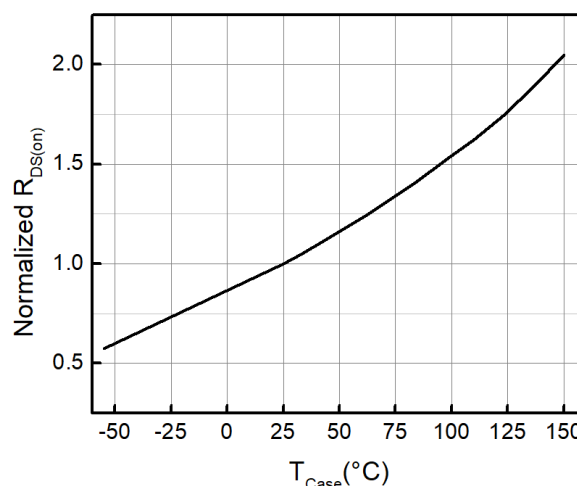
Figure 4. Normalized On-Resistance ( I_D = 22\text{A} , V_{GS} = 10\text{V} )
