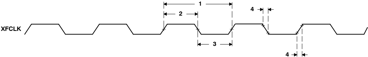
Figure 16. XFCLK Timings
