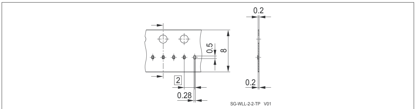
Figure 15 WLL-2-2 packing
