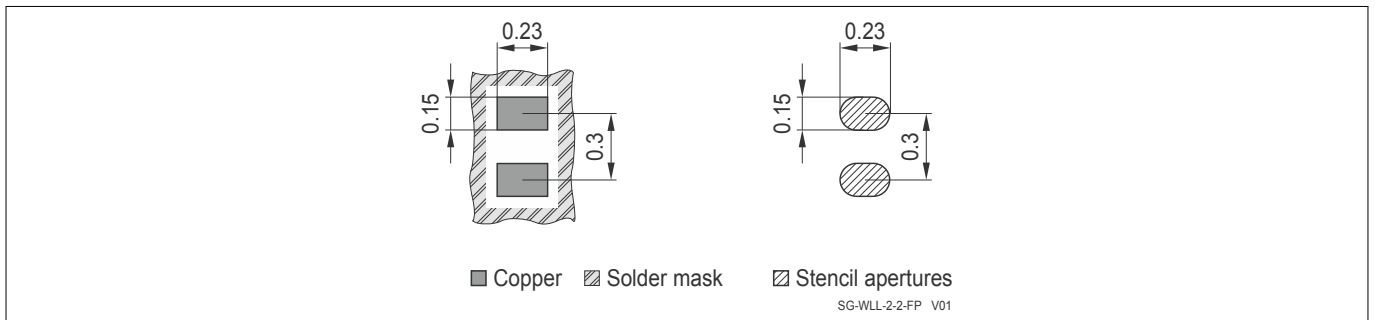
Figure 14 WLL-2-2 footprint
