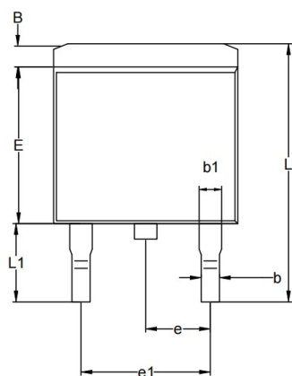
TOP VIEW [顶视图]
