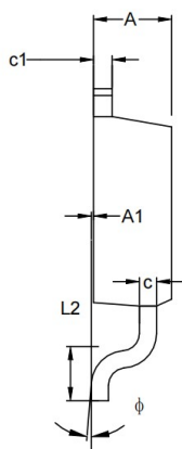
SIDE VIEW [侧视图]
