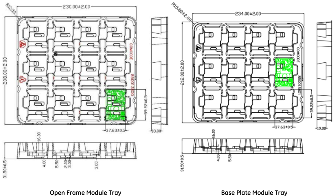
Figure 27. QBVW033 Packaging Tray
