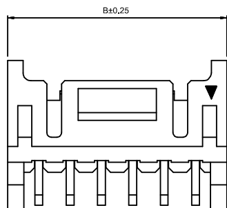
05P~13P Shape(Scale1:1)
