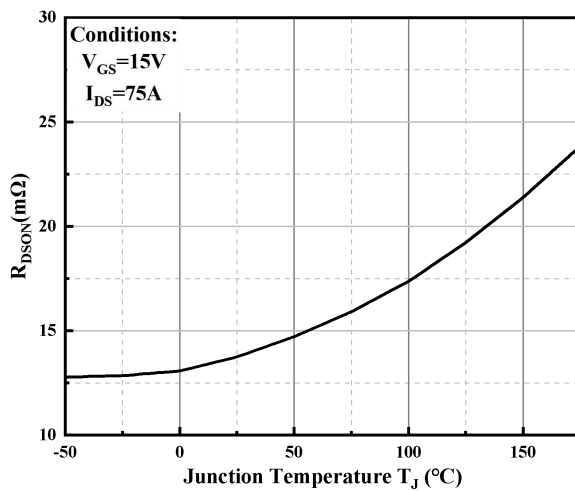
Normalized On-Resistance with Temperature
