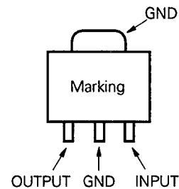
μPC78L00T Series
