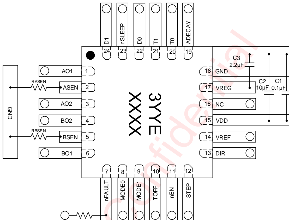
Figure 11 AW8646G External Components Placement
