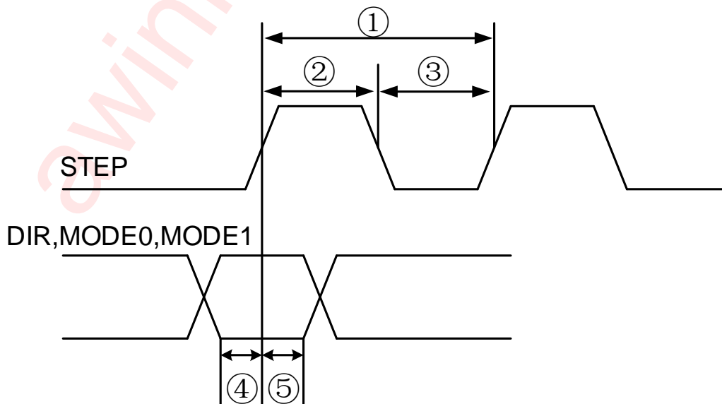
Figure 4 Timing Diagram
