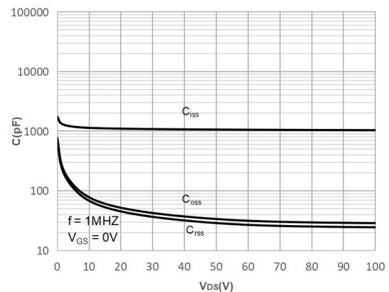
Figure 6: Capacitance Characteristics
