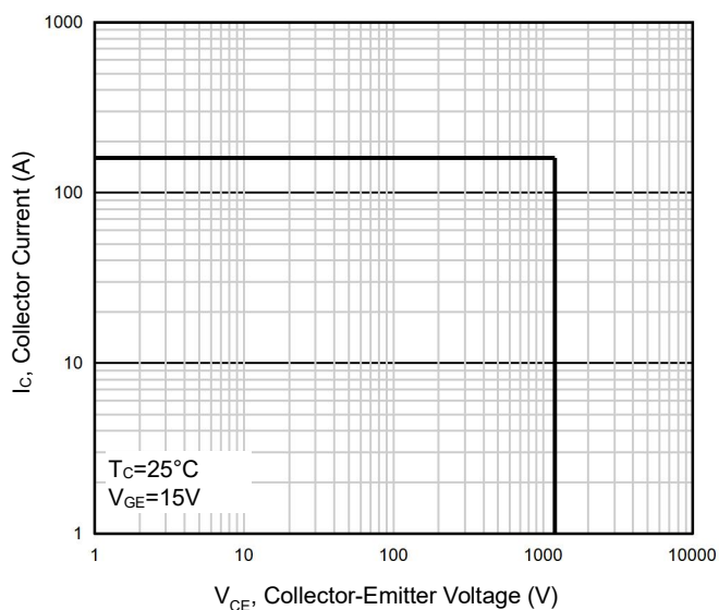
Figure 27 Reverse Bias SOA
