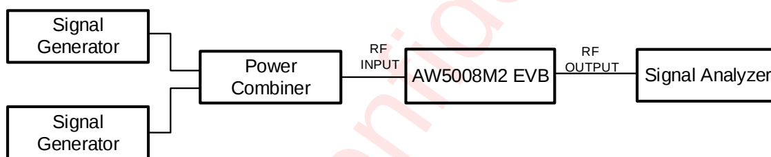
Figure 8 AW5008M2 IIP3 Measurement Diagram
