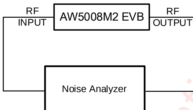
Figure 7 AW5008M2 Noise Figure Measurement Diagram
