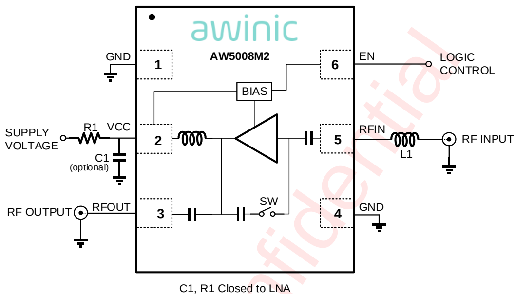
Figure 5 AW5008M2 DC Test Diagram
