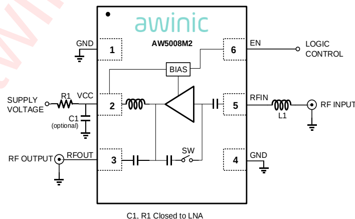
Figure 1 Typical Application Circuit of AW5008M2
