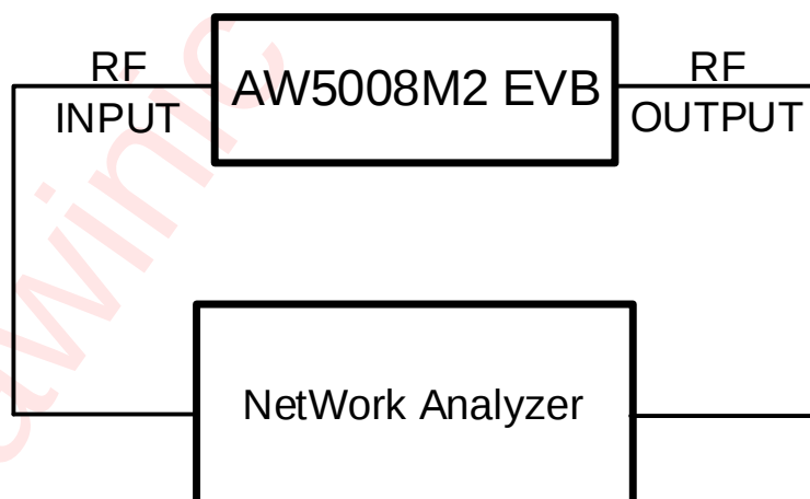
Figure 6 AW5008M2 S-parameter Measurement Diagram
