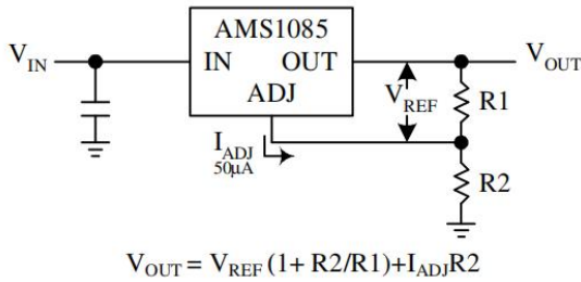
Figure 1. Basic Adjustable Regulator
