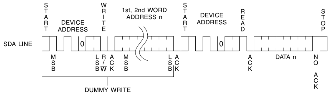
Figure 5. Random Read
