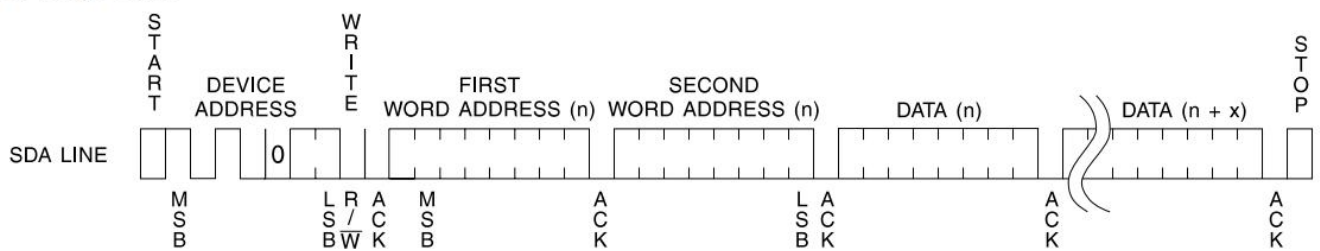
Figure 3. Page Write
