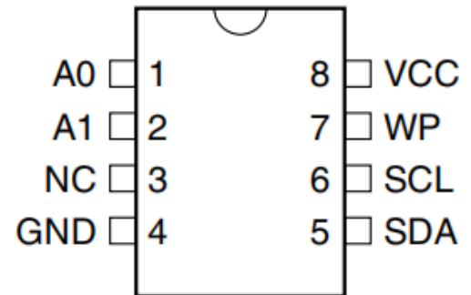
8-pin PDIP
