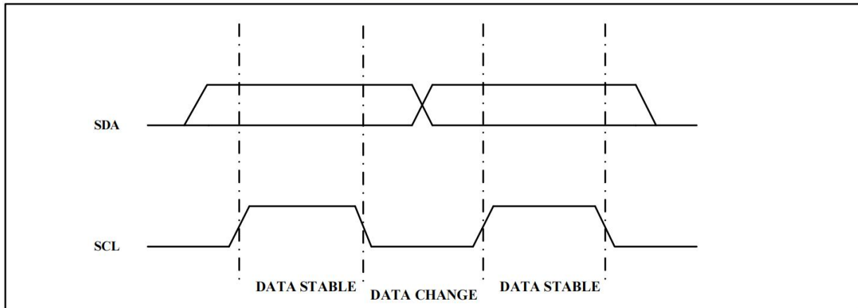
Figure 2. Data Validity
