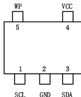
5-lead SOT23-5
