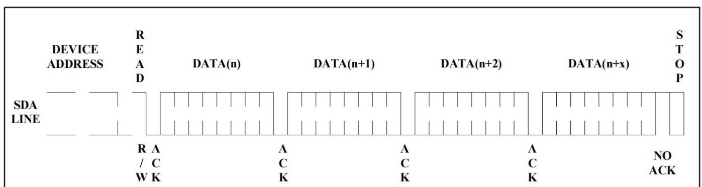
Figure 10. Sequential Read
