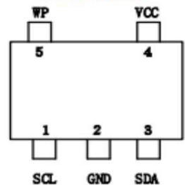
5-lead SOT23-5
