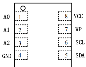
8-pad DFN
