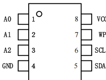
8-lead SOP
