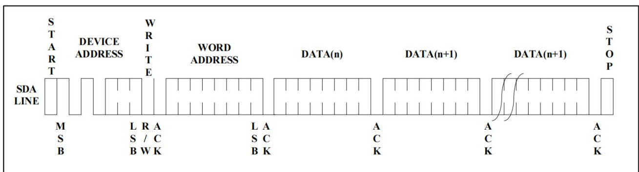
Figure 7. Page Write
