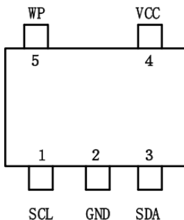
5-lead TSOT23-5
