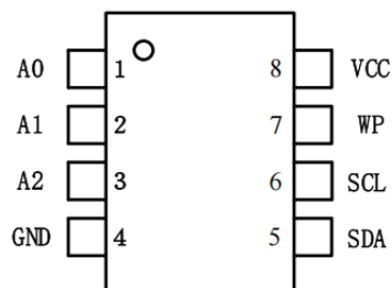
8-lead TSSOP
