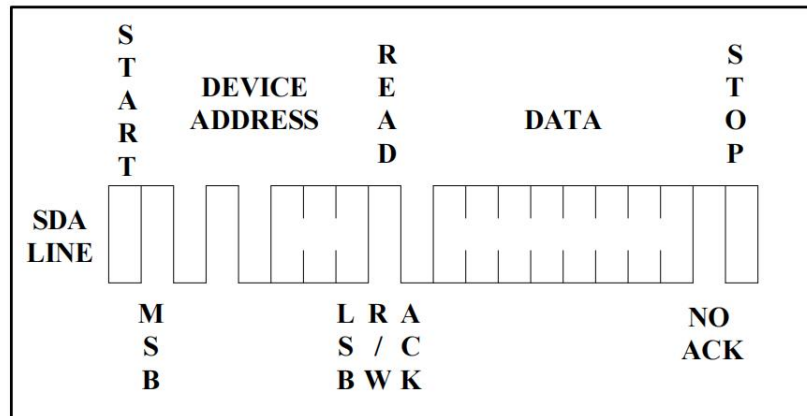
Figure 9. Random Read
