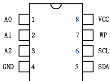
8-lead PDIP
