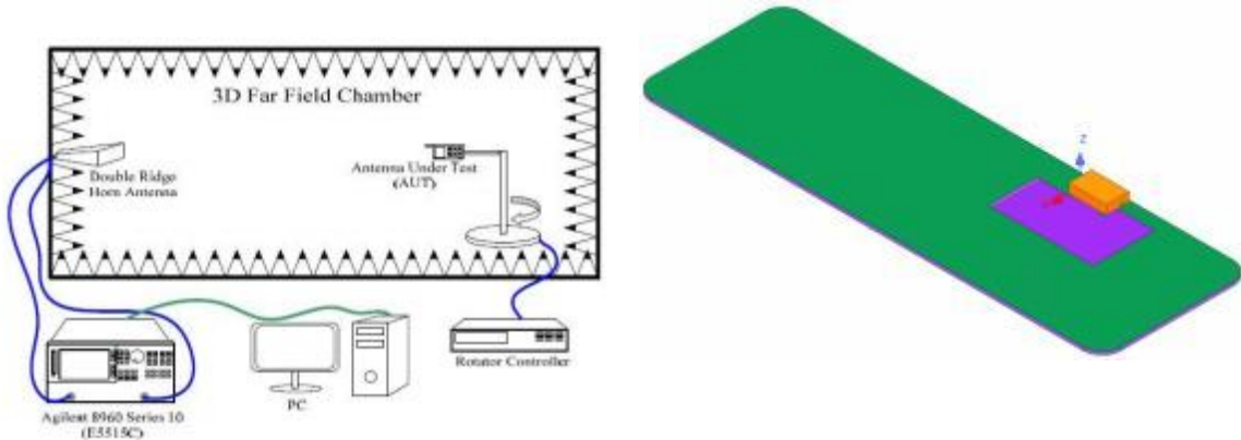
Fig.2 FAR-field Chamber
