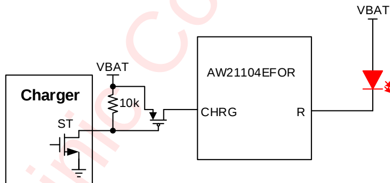
Figure 6 Real Charging Status Indication in Special Charger IC Application
