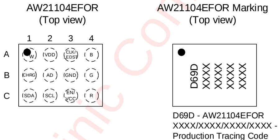
Figure 2 Pin Configuration and Marking
