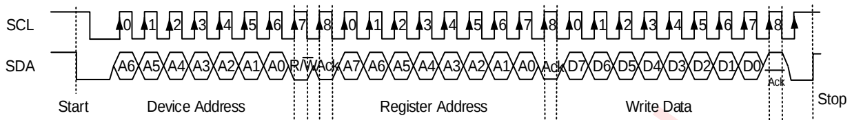
Figure 16 I²C Write Byte Cycle
