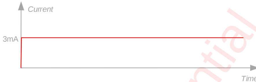
Figure 5 AW21104EFOR Auto Charging Indication Pattern Parameter
