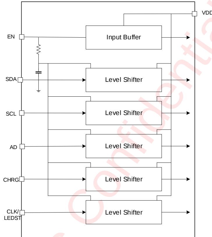
Figure 12 Using EN Pin as Digital I/O Voltage Reference
