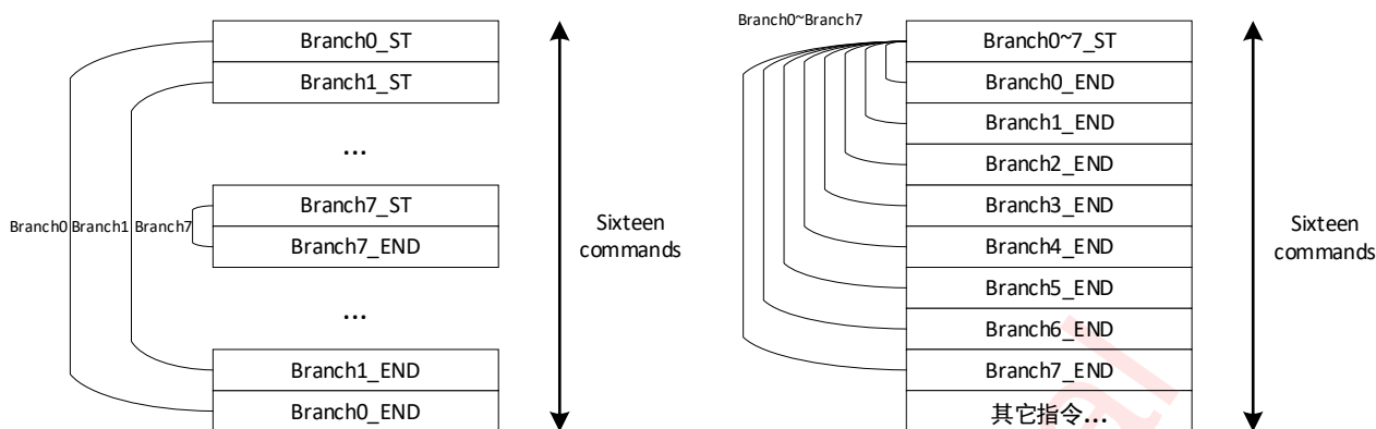
Figure 11 structure of maximum number nested loops
