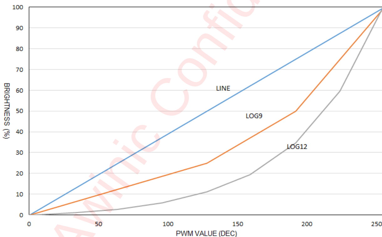
Figure 7 Logarithmic and Linear PWM Adjustment Curves
