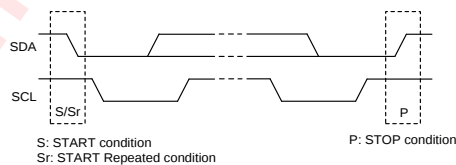
Figure 13 I 2 C Start/Stop Condition Timing
