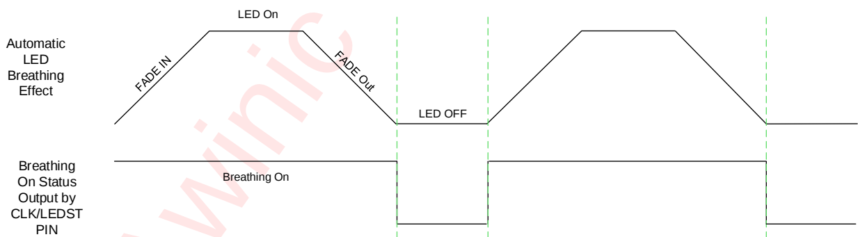
Figure 9 LED Status Indication Diagram
