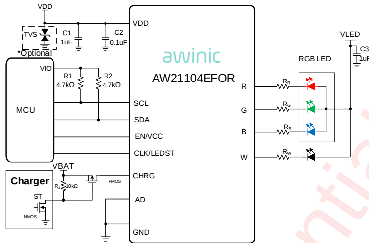
Figure 1 AW21104EFOR Simple Application Circuit
