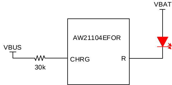
Figure 7 USB Power Insertion Status Indication in PMU-Controlled Charging Application
