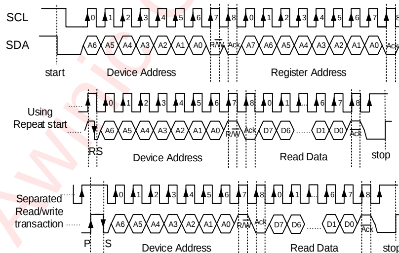
Figure 17 I²C Read Byte Cycle
