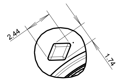
DETAIL B DIAMOND DOWEL SCALE 5:1
