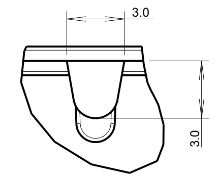
DETAIL A GATE CROSS-SECTION SCALE 5:1
