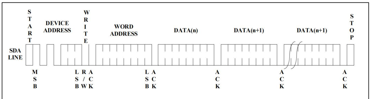
Figure 7. Page Write
