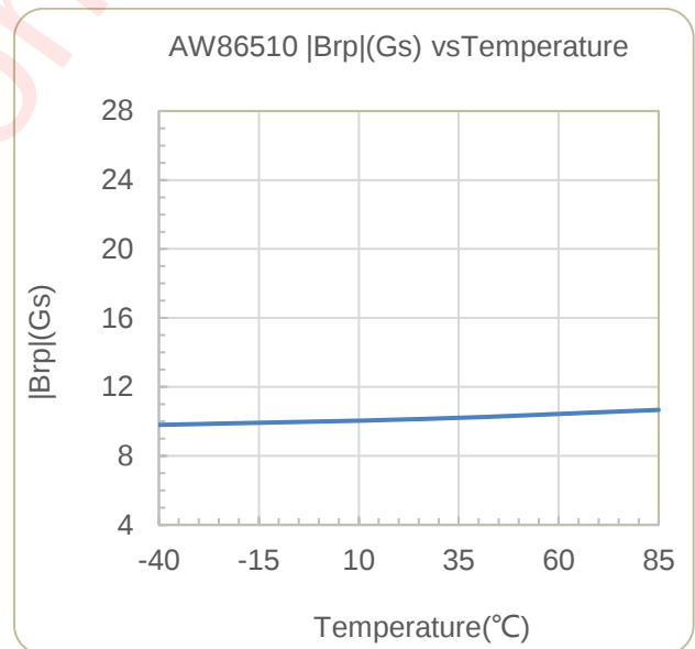
Ambient Temperature T_a [°C] |Brp| vs. T_a ( V_{DD}=3.3V )
