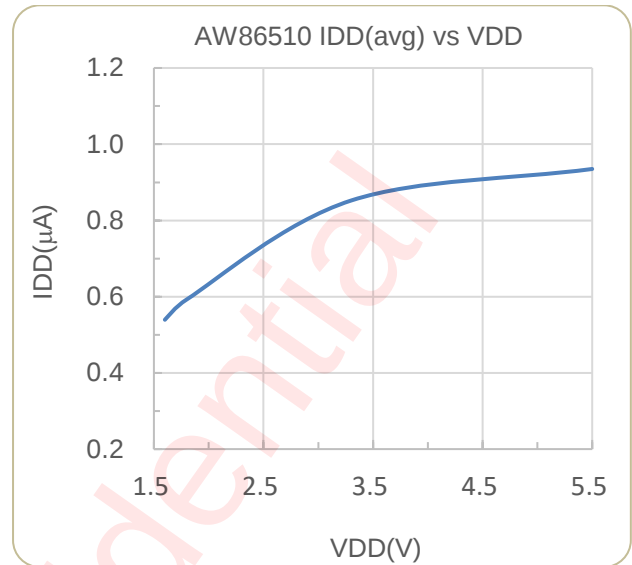
Average Supply Current vs. Supply Voltage ( T_a=25^{\circ}C )
