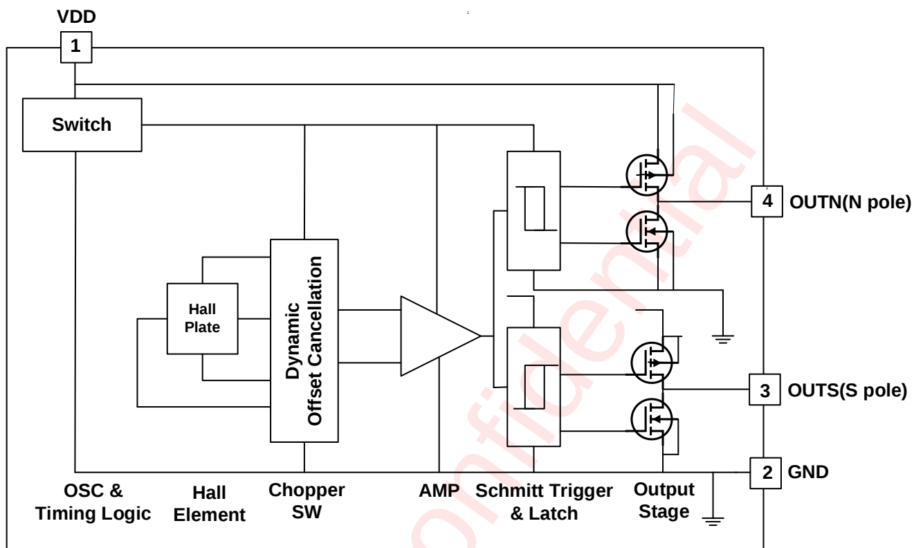
Figure 3 Functional Block Diagram of AW86510EU
