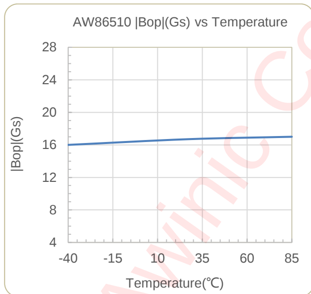
Ambient Temperature T_a [°C] |Bop| vs. T_a ( V_{DD}=3.3V )
