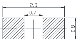
推荐焊盘尺寸 Recommended Soldering Pad
