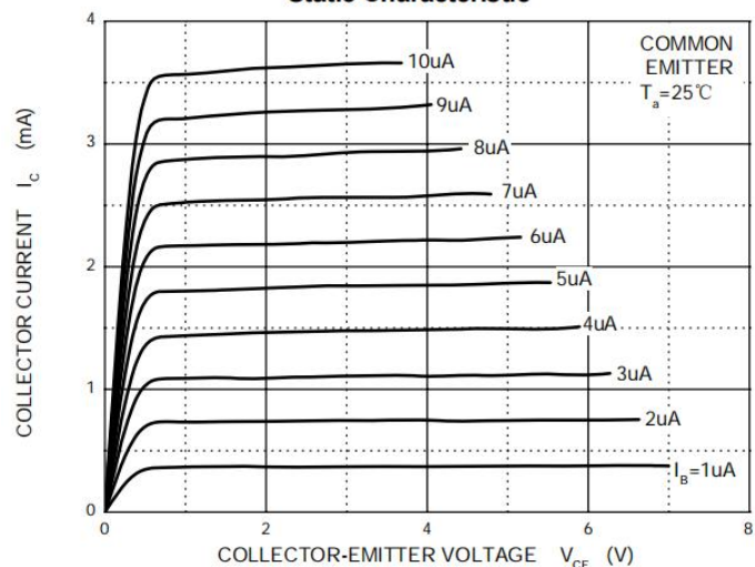
Static Characteristic
