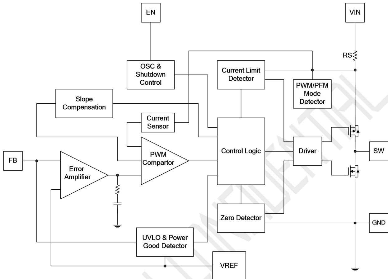
Figure 2. MT3410LB Block Diagram
