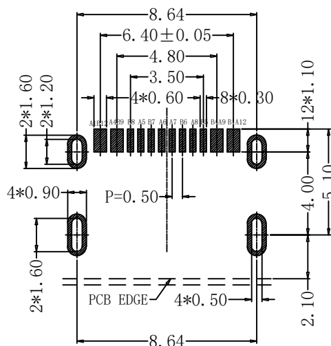
RECOMMENDED PCB LAYOUT TOP VIEW, TOL±0.05mm
