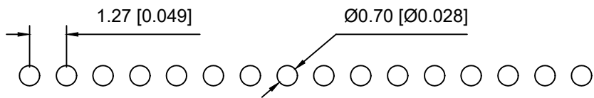
PCB LAYOUT
