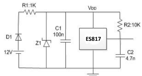
Automotive and Severe Environment Protection Circuit
